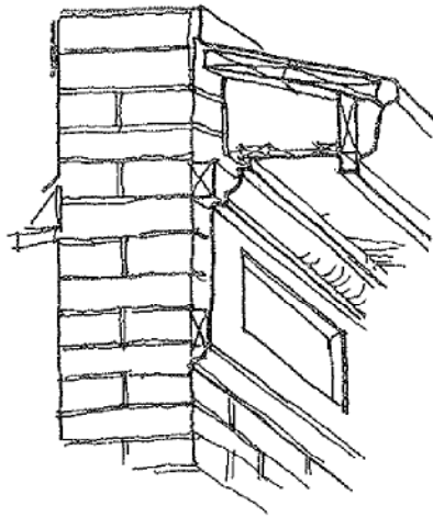
SHEET METAL CORNICE
